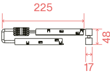
BI-EMISSION UP/DOWN ELECTRICAL CONNECTOR (REQUIRED - 1 KIT X LINEAR CONNECTION)
