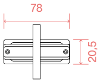
LINEAR CONNECTOR
